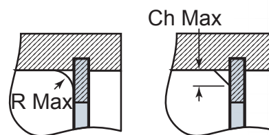
Maximum Corner Radius (R Max) & Chamfer (Ch Max) for Retained Part
